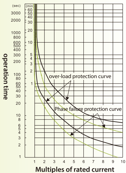
TH-P60TAPP tripping characteristic curve
