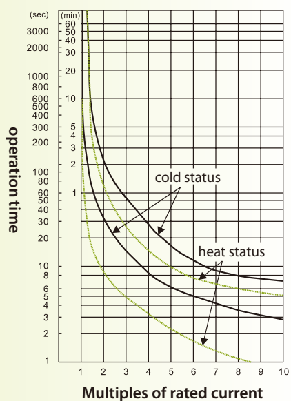
TH-P20ETA – above 9A tripping characteristic curve
