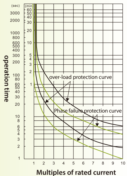
TH-P220CTPP、P400CTPP、P600CTPP、 TH-P220TPP、P400TPP tripping characteristic curve
