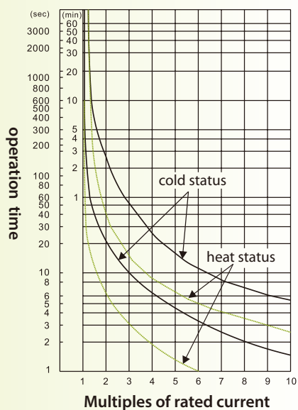
TH-P12E tripping characteristic curve
